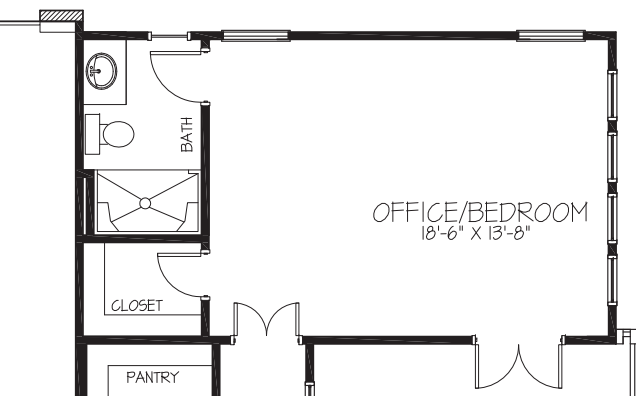
Optional Office/Bedroom extension with screened porch access
